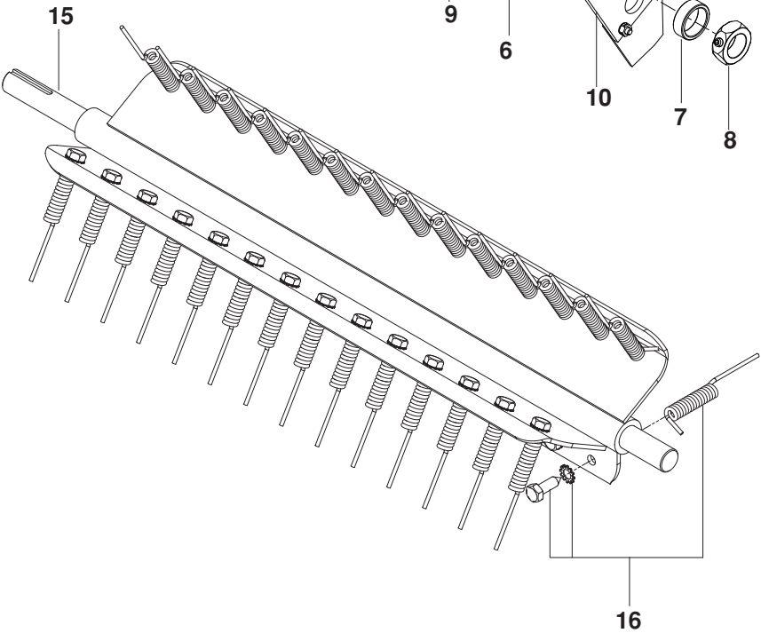
SPRING TINES
