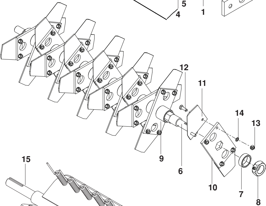
DELTA BLADE
